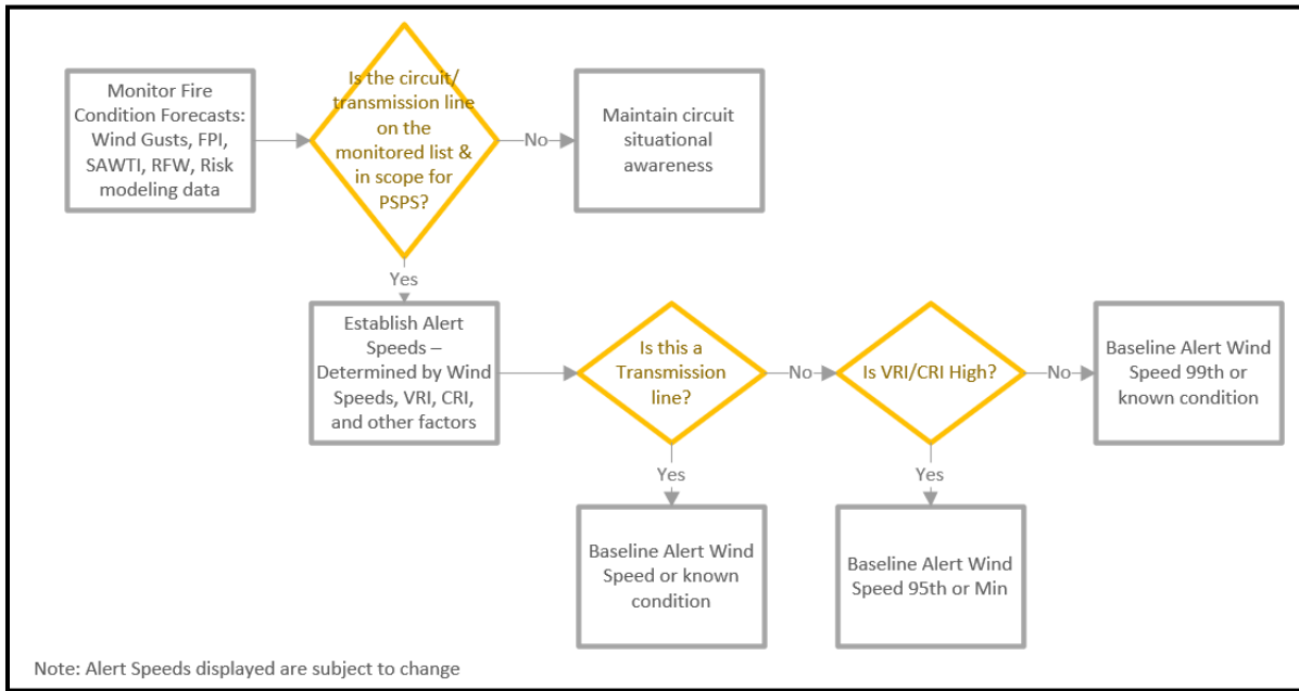
Figure 2: Alert Speed Calculation
