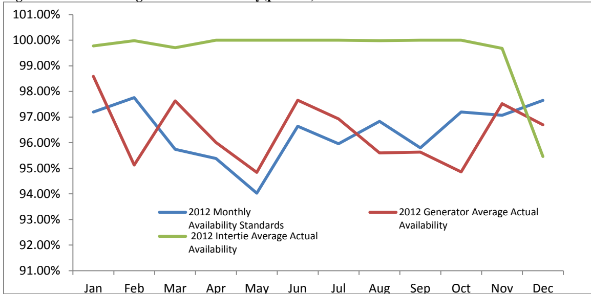
Figure 10. 2012 Average Actual Availability(percent)
